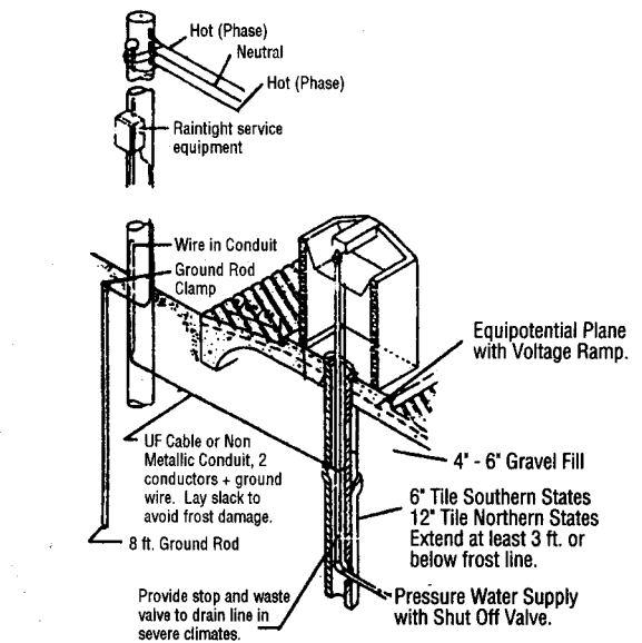
EXHIBIT C Waterer supplied by its own service equipment
