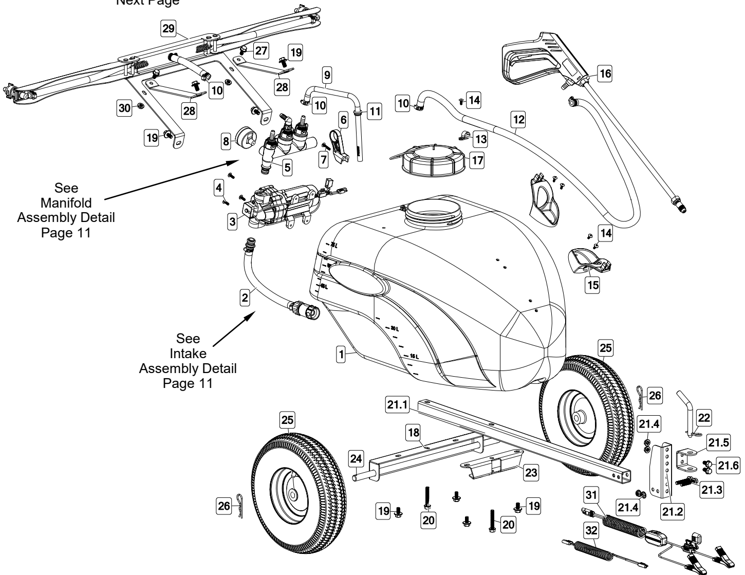
Exploded View/Parts List: LG-20-TRL (5302316)
