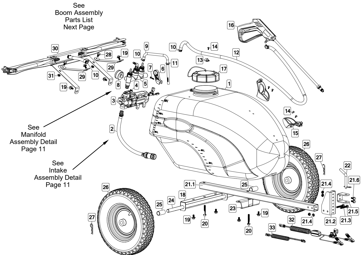
Exploded View/Parts List: LG-30-TRL (5302317)
