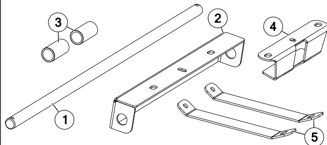
Bracket Kit LG-30-TRL (#5278366)
