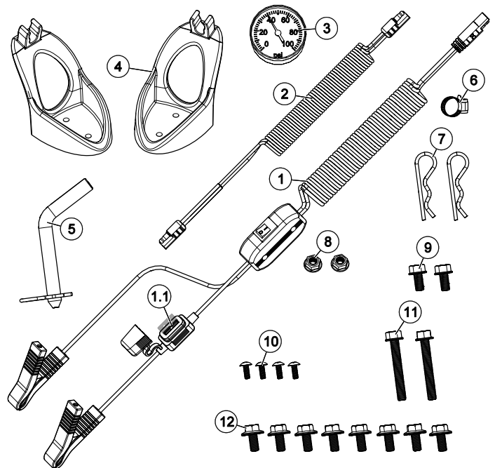
Contents of Parts Bag (#5278364)
